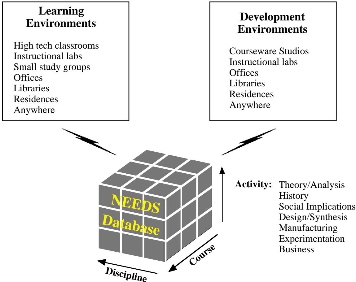
Fig. 1: The NEEDS database is linked to learning and development environments though the Internet. The database can be searched through a free text search and through a structured query. All courseware is cataloged in a modular fashion in order to capture the courseware curriculum dimensions shown above and allow reuse of courseware elements in other courseware.
